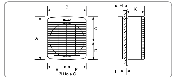
Dimensions (mm)
